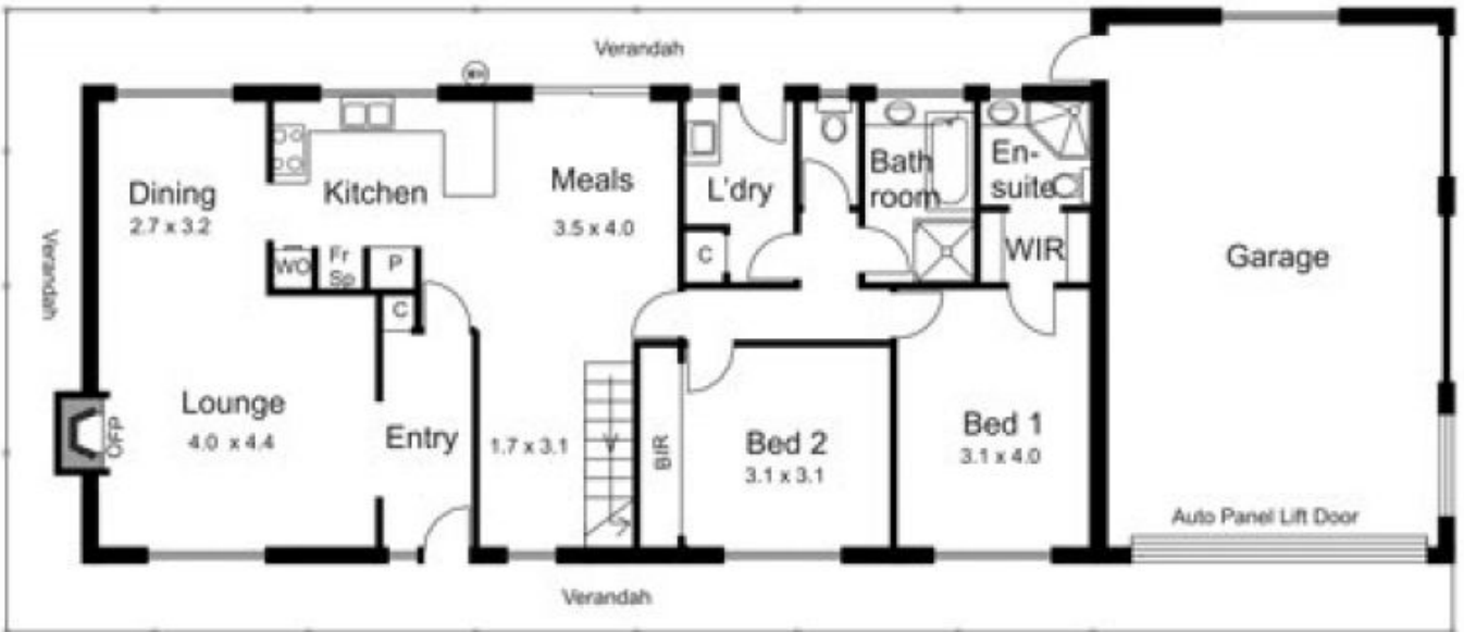
GROUND FLOOR
